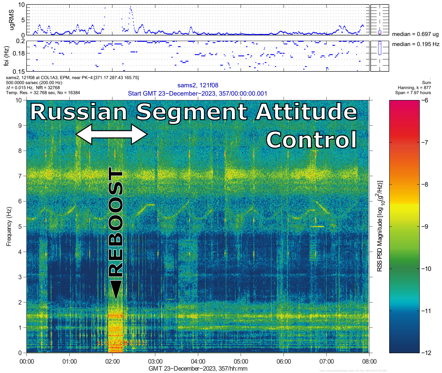
Fig. 2: 10 Hz Spectrogram showing Progress 85P Reboost on GMT 2023-12-23 from a SAMS Sensor in Columbus Module.
